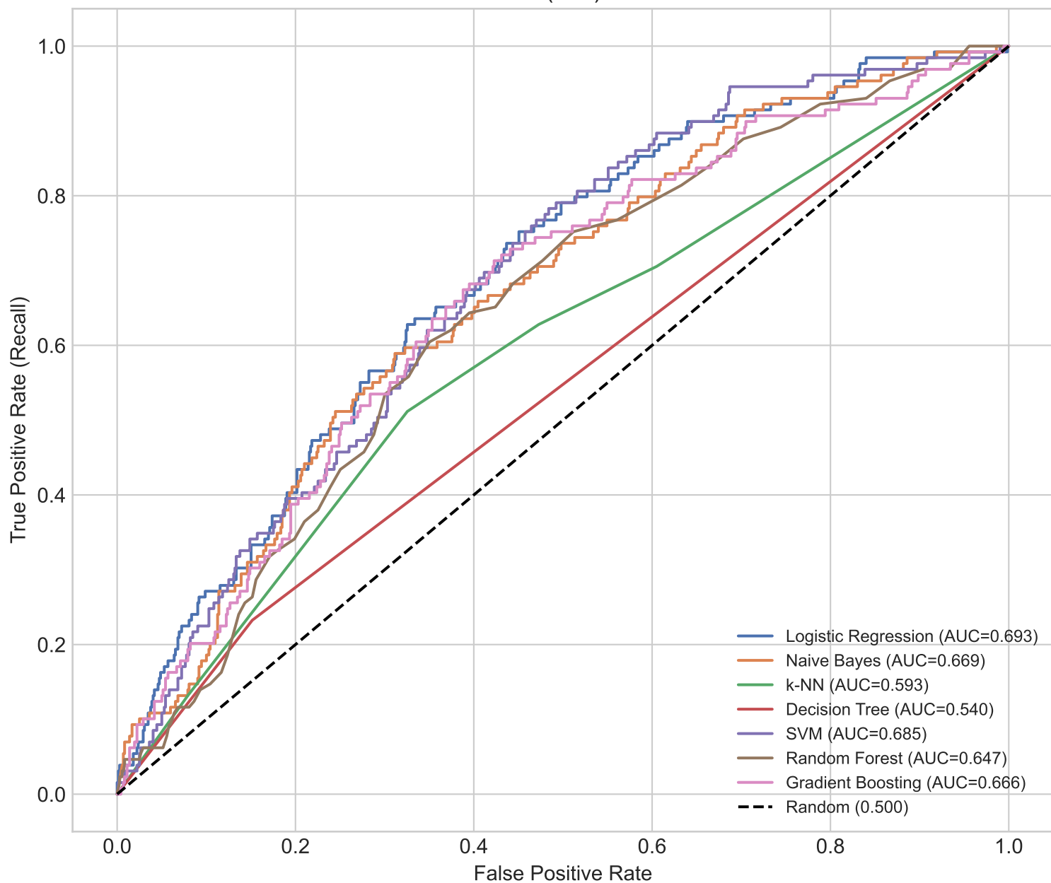
ROC curves (test) - unscaled
